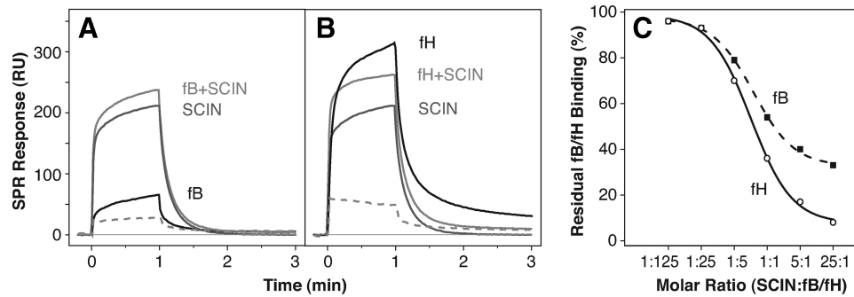
FIGURE 4. SCIN competes with fB and fH for binding to C3b. In an SPR experiment, constant concentrations (500 nM) of either fB (A) or fH (B) in HBS-Mg buffer were injected to immobilized C3b either alone (black line) or as mixtures with increasing concentrations (20 nM–12.5 \mu M) of SCIN (light gray line). The same dilution series of SCIN alone (dark gray line) was injected and subtracted from the corresponding signal of the fB plus SCIN mixture (dashed curve). For reasons of simplicity, the plots show only one concentration of SCIN (2.5 \mu M) and fB or fH (500 nM). C, The residual signals for both competition series were divided by the uninhibited fB or fH response and plotted against the molar ratio between SCIN and fH or fB concentrations. Although both complement factors compete with SCIN for binding to C3b, the effect is significantly more pronounced for fH than fB. A schematic representation of the assays is available (see supplemental Fig. S6, E and F). 5
