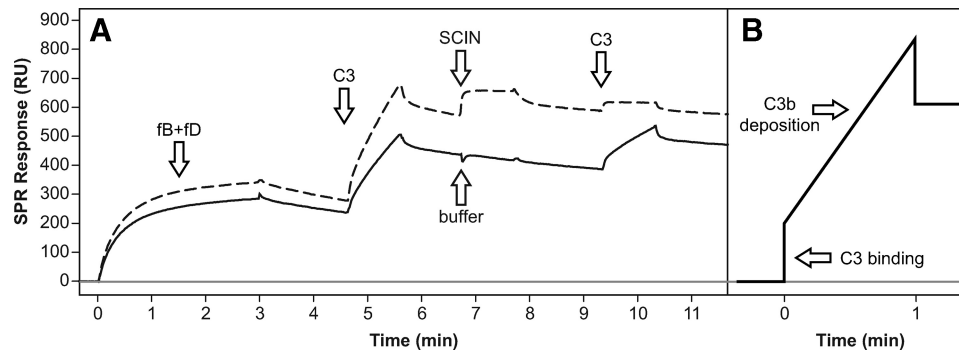
FIGURE 7. SCIN prevents C3 cleavage and C3b deposition by the C3 convertase. A , In a first cycle (solid curve), the C3 convertase was formed by injecting fB plus fD over immobilized C3b. When native C3 was injected, an initial sharp signal increase corresponding to C3 binding to the convertase and a slower binding slope representing deposition of cleaved C3b on the sensor chip surface could be observed (see schematic representation in panel B ). After a buffer injection, C3 was injected again and a similar yet smaller slope could be detected (due to the regular decay of the convertase). In a subsequent cycle (dashed curve), a higher convertase formation rate was observed due to the previously deposited C3b. Again, injection of C3 led to binding of C3 and deposition of cleaved C3b. However, after SCIN was injected to the convertase, only C3 binding but no deposition of cleaved C3b was detected, therefore indicating that SCIN prevented the activation of C3 to C3b by the convertase. A schematic representation of the assays is available (see supplemental Fig. S6J). 5
