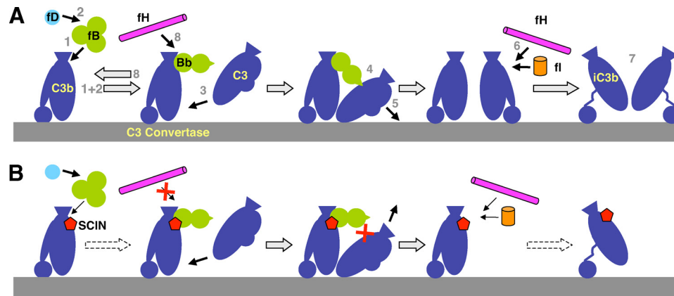
FIGURE 8. Potential effects of SCIN on complement activation and regulation. A , During normal complement activation, fB binds to C3b (1) and is converted to the C3 convertase (C3bBb) by fD (2). Native C3 binds to the convertase complex (3), becomes cleaved by Bb (4), and the resulting C3b is deposited on the surface (5). Surface-bound C3b can again participate in convertase formation (self-amplification) or can be degraded by fI and fH (6) to iC3b, which does not bind fB but is still involved in signaling (7). Finally, fH also regulates complement activity by accelerating the decay of the C3 convertase (8). B , By binding at a focal point on C3b, SCIN seems to interfere with this response in various ways: it slows down convertase formation but kinetically stabilizes the convertase complex in a state in which C3 can still bind but does not get cleaved. It also impairs the actions of fH by preventing decay acceleration and potentially decelerating the degradation to iC3b.
