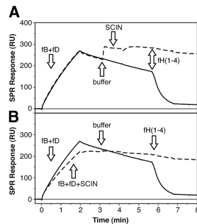
FIGURE 6. SCIN influences the formation, decay, and stability of the alternative pathway C3 convertase. A, The on-chip formation and decay of the C3 convertase was established by injecting a 1:1 mixture of fB and fD (100 nM each) onto immobilized C3b using SPR (solid curve). After injection end (2 min), a moderate decay of the convertase could be observed, which was greatly accelerated upon injection of fH(1–4) (1 \mu M). When SCIN (1 \mu M) was injected after formation of the convertase (dashed curve), the inhibitor bound to the complex, slowed the decay rate, and impaired the decay accelerating action of fH(1–4). B, When SCIN (1 \mu M) was added to the fB plus fD mixture, it partially reduced the formation of the C3bBb complex, and showed the same effect on the stability and fH(1–4) resistance as in A. A schematic representation of the assays is available (see supplemental Fig. S6H). 5
