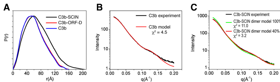
FIGURE 2. SCIN and C3b form a mixture of monomeric and dimeric complexes when analyzed by SAXS. A , Pair-distance distribution function ( P(r) ) calculated for scattering data collected on solutions of C3b-SCIN (black), C3b-ORF-D (red), and C3b alone (blue). Note the shift in r(\text{Å}) value, where pair-distance distribution function is maximal and the long-tailing pair-distance distribution function curve for C3b-SCIN relative to the control samples. B , Experimental scattering curve of unliganded C3b observed in solution (black) compared with the theoretical scattering curve for an unliganded C3b crystal structure (PDB code 2I07 (29)). C , Guinier analysis of the C3b-SCIN experimental data as compared with theoretical scattering curves for a sample comprised entirely of C3b dimer (green) or 40/60 percentage C3b dimer to C3b monomer (red), as determined by the program OLIGOMER (28). The value for the quality of fit parameter ( \chi^2 ) is shown in B and C .
