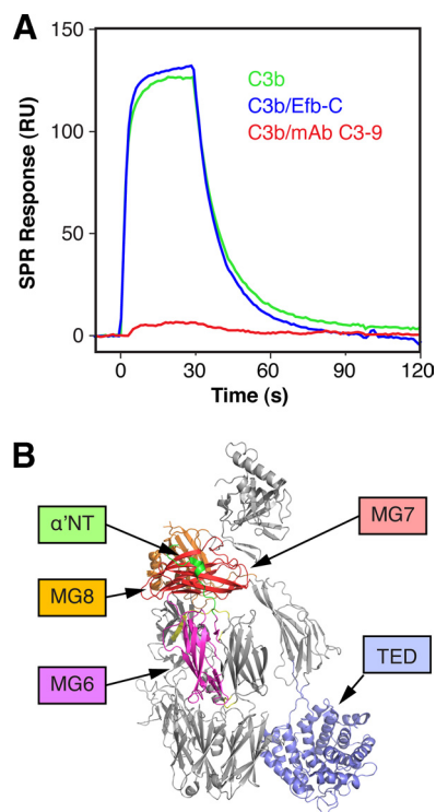
FIGURE 3. The SCIN binding site can be localized at a functionally important area on C3b. A , The binding of SCIN to immobilized C3b was compared in the presence or absence of mAb C3–9 (anti-C3c) and the bacterial complement inhibitor Efb-C. Whereas SCIN bound similarly well to the C3b-Efb-C complex (blue) compared with free C3b (green), mAb C3–9 led to a significant decrease in binding activity (red). B , The domains involved in binding of mAb C3–9 (MG7, MG8 (32)), Efb-C (TED (10)), and the fragment fH(1–2), and Ba ( \alpha' NT, MG6, MG7 (18)) have been highlighted on the crystal structure of C3b (PDB code 2I07 (29)). A schematic representation of the assays is available (see supplemental Fig. S6D). 5
