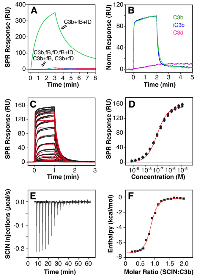
FIGURE 1. SCIN binds to both surface-bound and solution-based C3b with nanomolar affinity. A , When SCIN was immobilized on a SPR chip surface, only the convertase mix (C3b plus fB plus fD) showed significant affinity. B , In contrast, solution-based SCIN (1 \mu\text{M} ) bound with similar activity to C3b (green) and iC3b (blue) that have been immobilized via their thioester moiety to the SPR sensor chip. No significant binding was observed for C3d (magenta). C , The binding mode and affinity of SCIN was further elucidated using SPR by injecting a dilution series of SCIN (0.8 nM–12.5 \mu\text{M} ) to site-specifically immobilized C3b. Despite some heterogeneity at higher concentrations, the interaction featured reproducible triplicate injections (black SPR signals) and fitted reasonably well to a Langmuir 1:1 kinetic model (red fitting curves). D , In agreement with the kinetic analysis, the steady state signals (black filled symbols) could be fitted to a single-binding site model and showed clear signs of saturation (red fitting curve). A direct interaction between SCIN and C3b was also detected in solution using ITC. E , Injection of SCIN (120 \mu\text{M} ) into C3b (12 \mu\text{M} ) produced a dose-dependent, exothermic response. F , The integrated data (filled black symbols) could be fitted to a single set of sites (red fitting curve). RU, Resonance units. A schematic representation of the assays is available (see supplemental Fig. S6, A–C). 5
