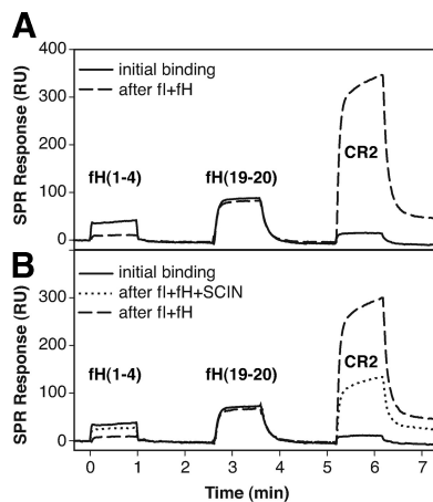
FIGURE 5. SCIN inhibits the cofactor activity of fH. A, The fI-mediated degradation of surface-bound C3b by fI was observed by using SPR with fH(1–4) as a probe for intact C3b and CR2 for degraded C3b (i.e., iC3b). fH(19–20) was used as a control that is not affected by the cleavage. After sequential injection of the three probes over intact C3b (solid curve), a degradation mixture of fI plus fH was injected, and the probes were assessed again (dashed curve): degradation of C3b to iC3b was manifested in an impairment of fH(1–4) binding with a simultaneous increase in CR2 activity. B, The SPR experiment in A was repeated with the same degradation mixture in presence of SCIN. Injection of this mixture led only to a partial degradation with significantly lower effects on fH(1–4) and CR2 (dotted curve). When the degradation mixture was injected in absence of SCIN, full degradation could be achieved again (dashed curve). A schematic representation of the assays is available (see supplemental Fig. S6G). 5
