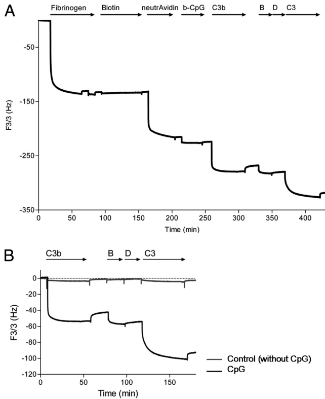
FIGURE 5. CpG 2006 facilitates AP convertase build-up. QCM-D was used to study the interaction of CpG 2006 with C3b. A , A gold sensor was covered with fibrinogen that was biotinylated in the QCM chamber. Subsequently, NeutrAvidin and biotinylated CpG were added. After that, C3b was injected and incubated. Then the AP convertase was built up using factors B, D, and C3. Each step was followed by washing (except after factors B, D, and C3). Frequency as well as dissipation (not shown) were monitored over time. B , C3b binding reflected by a drop in frequency that corresponds to mass increase on the sensor (black line). Control experiment (gray line) where biotinylated CpG 2006 was omitted in the surface build-up is shown. Normalized frequency was extracted from the third overtone. One representative experiment out of two is shown.
