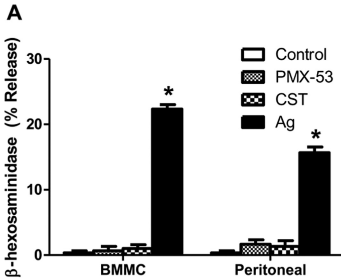
Fig. 8. PMX-53 and CST do not activate murine peritoneal and bone marrow-derived mast cells. A, murine bone marrow-derived and peritoneal mast cells were incubated with DNP-specific mouse IgE (1 \mu g/ml, 16 h). Cells were exposed to buffer (control), 1 \mu M PMX-53, 1 \mu M CST, or 30 ng/ml DNP-BSA (Ag) for 30 min, and \beta -hexosaminidase release was measured. Data are mean \pm S.E.M. of n = 3 . B, murine bone marrow-derived mast cells were incubated with DNP-specific mouse IgE (1 \mu g/ml, 16 h). Cells were incubated with Indo-1AM and were exposed to 1 \mu M PMX-53, 1 \mu M CST, or 100 ng/ml DNP-BSA, and intracellular Ca^{2+} mobilization was determined. Data shown are representative of three similar experiments. Statistical significance was determined by one-way ANOVA with Dunnett's post test. *, p < 0.05 .
