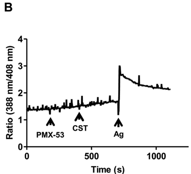
Fig. 8. PMX-53 and CST do not activate murine peritoneal and bone marrow-derived mast cells. A, murine bone marrow-derived and peritoneal mast cells were incubated with DNP-specific mouse IgE (1 \mu g/ml, 16 h). Cells were exposed to buffer (control), 1 \mu M PMX-53, 1 \mu M CST, or 30 ng/ml DNP-BSA (Ag) for 30 min, and \beta -hexosaminidase release was measured. Data are mean \pm S.E.M. of n = 3 . B, murine bone marrow-derived mast cells were incubated with DNP-specific mouse IgE (1 \mu g/ml, 16 h). Cells were incubated with Indo-1AM and were exposed to 1 \mu M PMX-53, 1 \mu M CST, or 100 ng/ml DNP-BSA, and intracellular Ca^{2+} mobilization was determined. Data shown are representative of three similar experiments. Statistical significance was determined by one-way ANOVA with Dunnett's post test. *, p < 0.05 .
