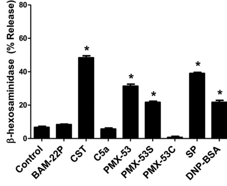
Fig. 7. PMX-53 uses MrgX2 to induce mast cell degranulation. RBL-2H3 cells stably expressing MrgX1 (A) or MrgX2 (B) were incubated with anti-DNP specific IgE (1 \mu g/ml, 16 h) and stimulated with the indicated peptides (1 \mu M), substance P (SP; 1 \mu M), or antigen (DNP-BSA; 30 ng/ml) for 30 min, and \beta -hexosaminidase release was measured. C and D, MrgX1 and MrgX2-expressing cells were also incubated with Indo-1AM and stimulated with selected peptides (1 \mu M), and intracellular calcium mobilization was determined. Data shown are representative of three similar experiments. Statistical significance was determined by one-way ANOVA with Dunnett's post test. *, p < 0.05 .
