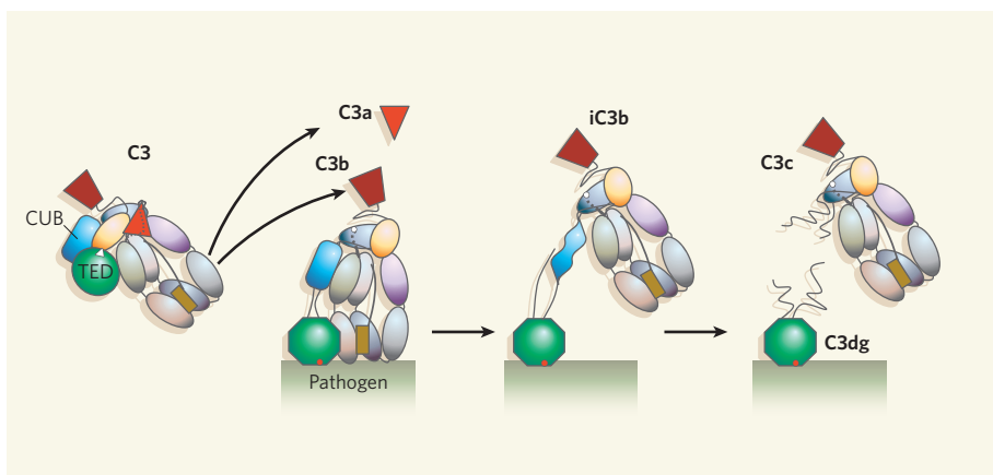
Figure 2 | Breakdown of complement C3. This model is based on the structures reported by Janssen et al. 3 , Ajees et al. 4 and Wiesmann et al. 5 . Cleavage of native C3 protein by the enzyme C3 convertase releases C3a and induces a major shift in the overall conformation of the remaining C3b molecule. Full exposure of the thioester domain (TED) facilitates binding of the thioester (red dot) to a target pathogen surface. The opening up of C3b exposes binding sites for components of the alternative pathway such as factor B as well as regulators of complement such as factor H. These regulators aid the sequential degradation of C3b to iC3b, C3c and C3dg. C3c is inactive, but each of the other split products has further functions in immunity.
