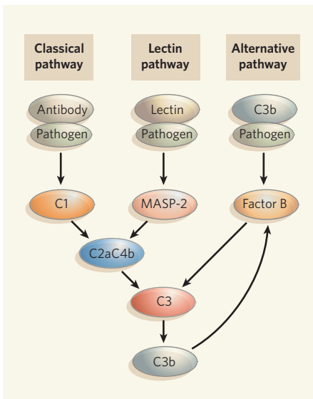
Figure 1 | Complement C3 is activated by three pathways. In the classical pathway, antibody bound to pathogen surface leads to the activation of C2aC4b. This is a 'convertase' enzyme that cleaves C3 into C3a and C3b — the active form (see also Fig. 2). Similarly, the lectin pathway is triggered following recognition of pathogens by the lectin protein, which binds to sugar molecules on their surface. This results in activation of the enzyme complex MASP2 (mannan associated serine protease 2) that forms the C2aC4b convertase. The alternative pathway not only amplifies the classical pathway and the lectin pathway but it can also be activated spontaneously. C3b bound to pathogen surfaces interacts with the blood serum protein factor B, which forms an alternative convertase called C3bBb.
